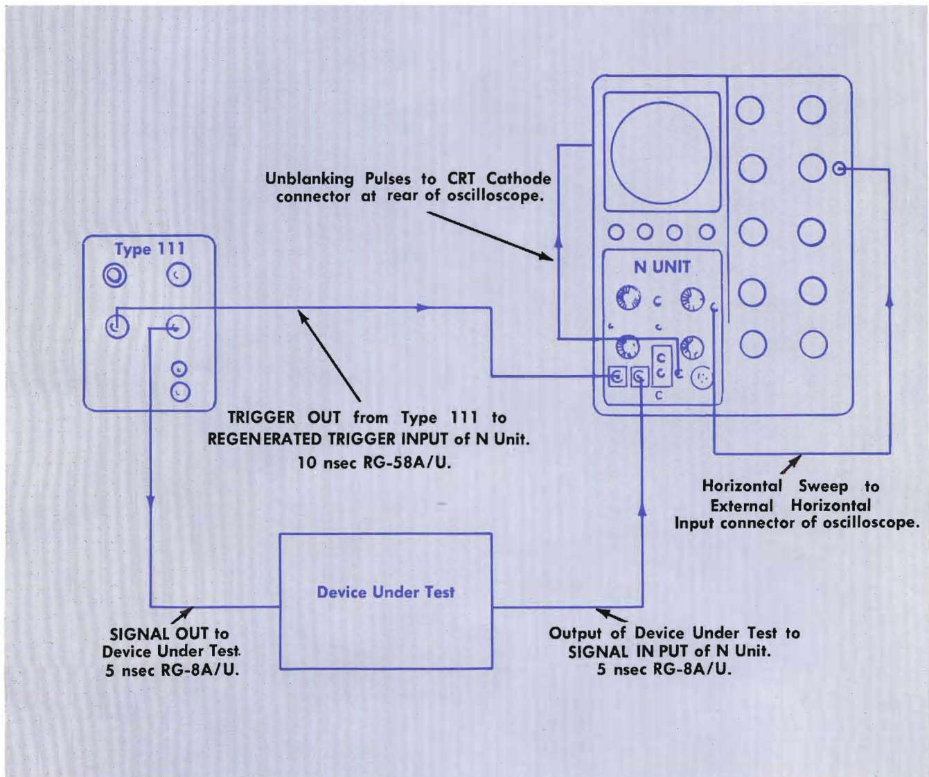
Fig. 2-4. Cable connections for the Type N Unit when used with the Type 111 Pretrigger Pulse Generator.
