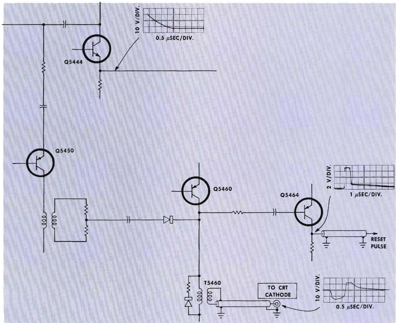
Fig. 5-1. Pulse Generator Channel output waveforms.
