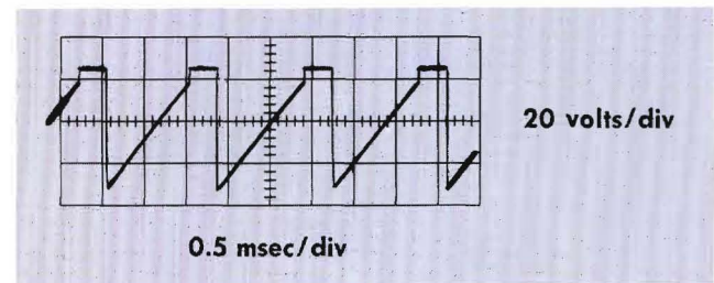
Fig. 5-6. Waveform at TO EXT. HORIZ. connector (SAMPLES/DISPLAY switch at 50).
